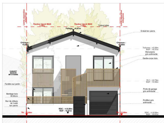
FACADE SUD
