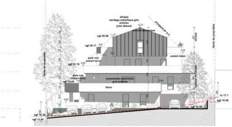
facade sud
